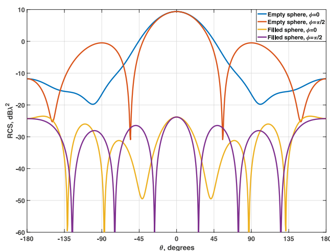
Figure 5. Comparison of the SCS for a silica sphere of \lambda_0 diameter empty and with the positive multilayer dielectric filler.
