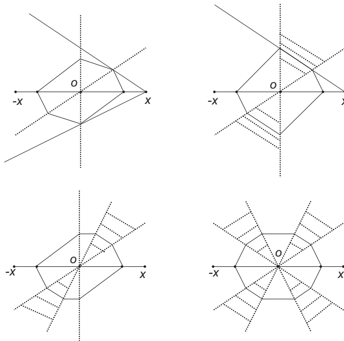
Figure 6: The asymptotes.
