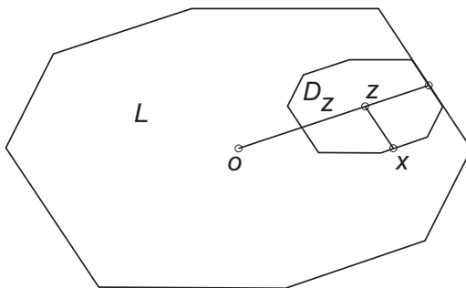
Figure 2: The equivalence of Definitions 1 and 2.
