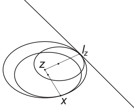
Figure 8: The case of strict convexity.
