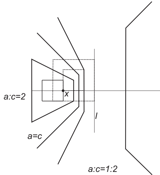
Figure 3: Conics in the l_\infty plane
