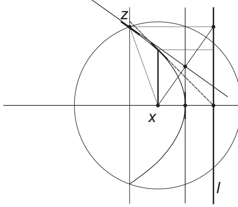
Figure 7: The Euclidean case.
