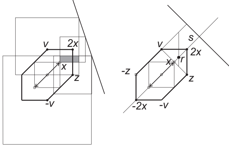
Figure 4: A metrical ellipse which has no leading line.
