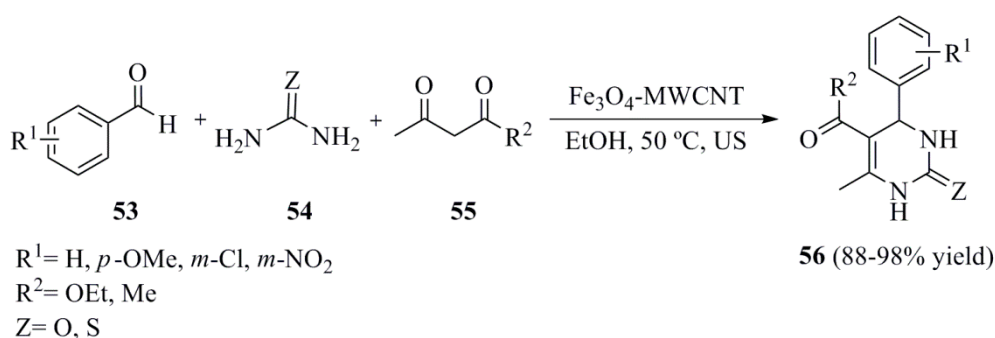
Scheme 16. Multicomponent synthesis of dihydropyrimidin-ones/thiones using \text{Fe}_3\text{O}_4 -MWCNT under ultrasonication.
