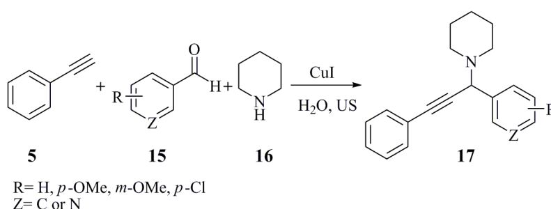
Scheme 6. Cu(I)-mediated synthesis of propargylamines.
