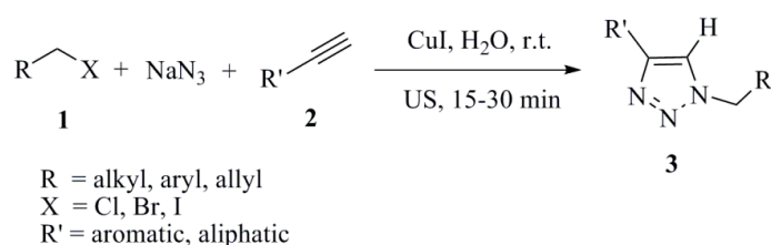
Scheme 1. Ultrasound-promoted three-component Cu-catalyzed alkyne-azide cycloaddition (CuAAC) in water.
