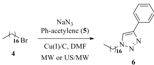
Scheme 2. CuAAC reaction activated by microwaves (MW) or simultaneous microwave-ultrasound (MW/US) irradiations.
