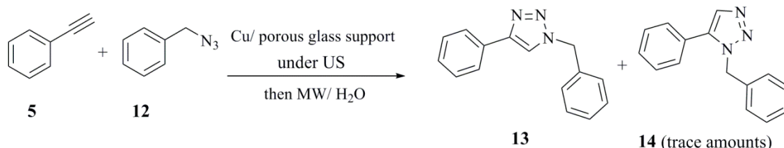
Scheme 5. Click-reaction using a porous glass support.
