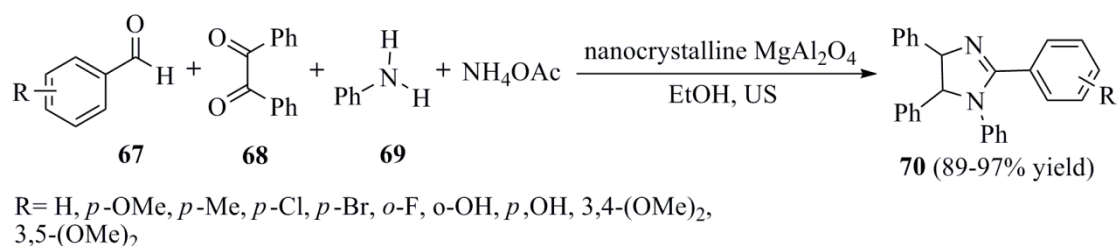
Scheme 22. Ultrasound-promoted synthesis of 1,2,4,5-tetrasubstituted imidazoles mediated by Mg/Al NPs.
