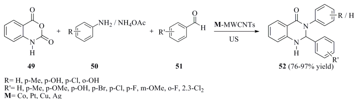
Scheme 15. One-pot multicomponent condensation catalyzed by metal multi-walled carbon nanotubes (MWCNTs) under ultrasound irradiation.
