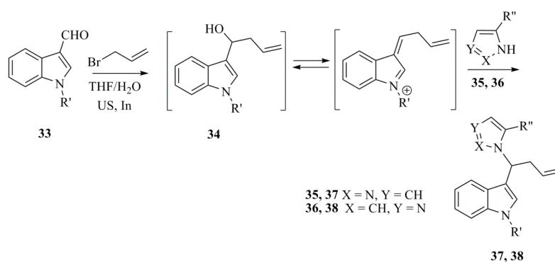
Scheme 11. Indole syntheses involving Barbier allylindation promoted by sonication.
