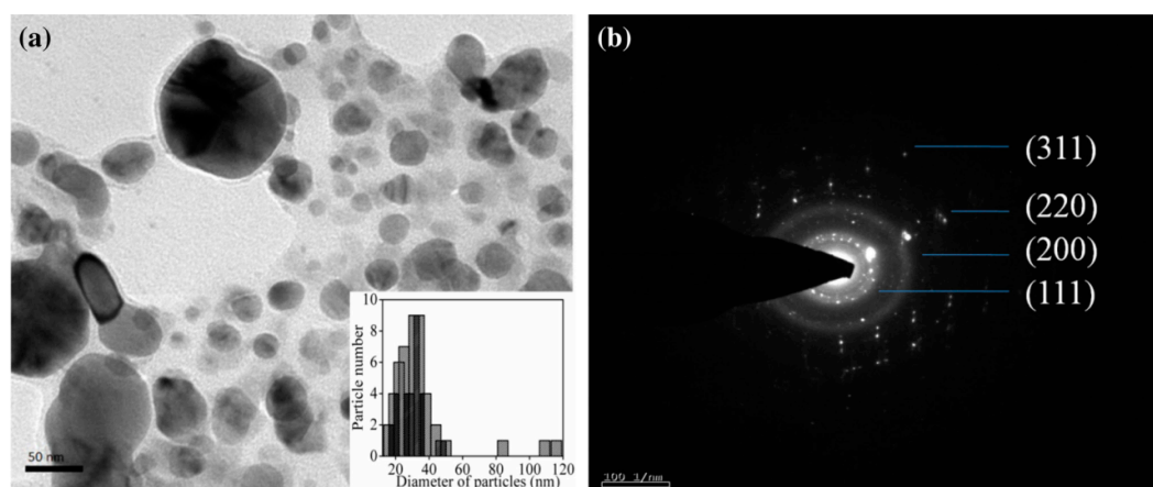
Figure 3. (a) TEM (transmission electron microscopy) images of Ag-NPs generated from Lantana camara L. extract under ultrasound. The box shows the resulting particle size distribution; (b) SAED (selected area electron diffraction analysis) pattern. Reproduced with permission from Ref. [94]. Copyright 2016 Springer.
