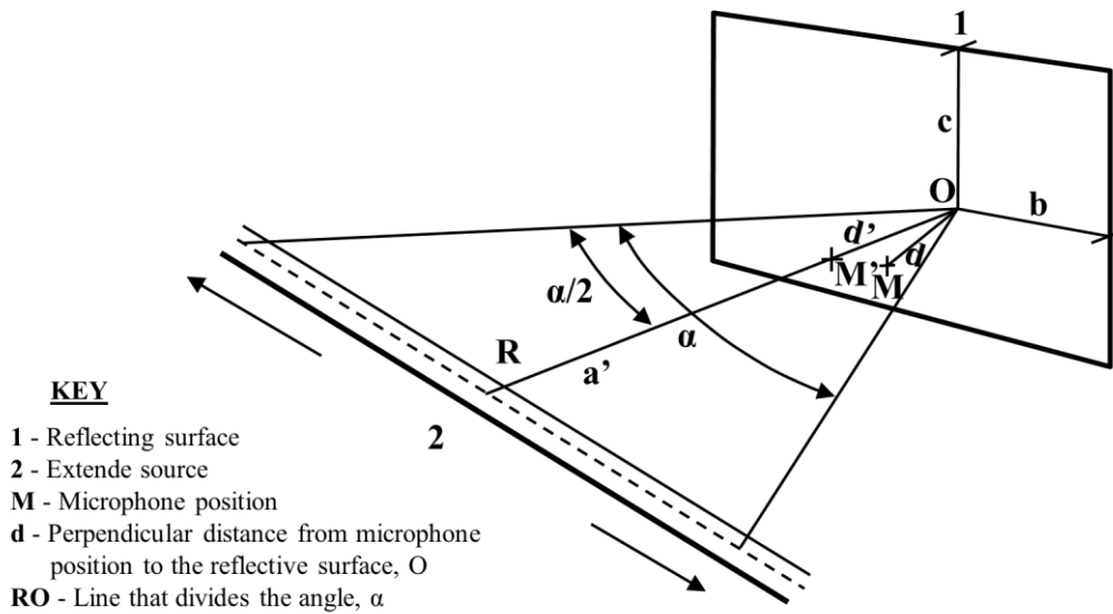
Fig. 1. Microphone near the reflecting surface (ISO 1996-2, 2007)
