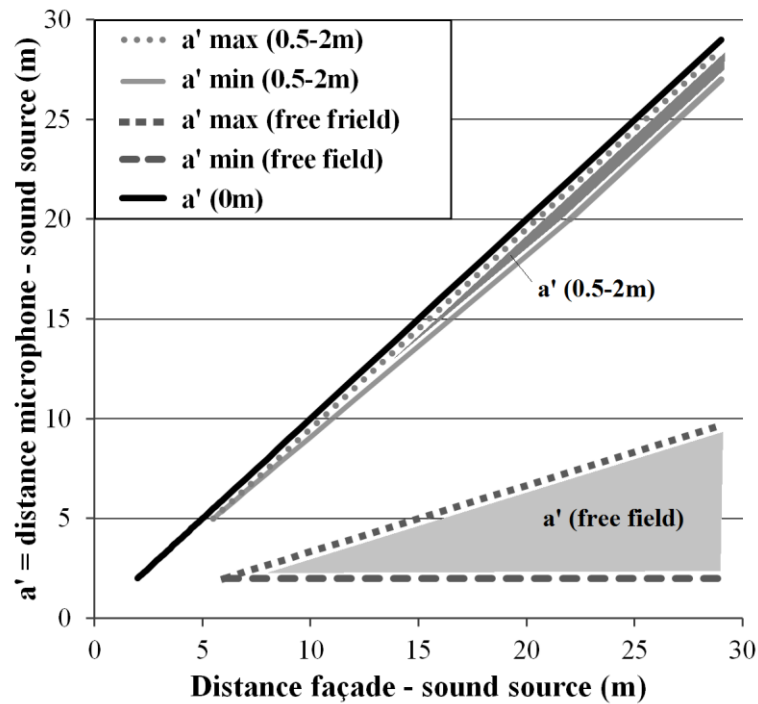
Fig. 2. Relationship between the distances façade-microphone and façade-sound source (a) and relationship between the distances microphone-sound source and facade sound-source (b) according to the measurement areas regulated in Annex B (informative) of ISO 1996-2 standard
