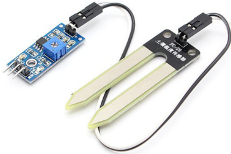
Fig. 5.4: FC-28 humidity sensor
