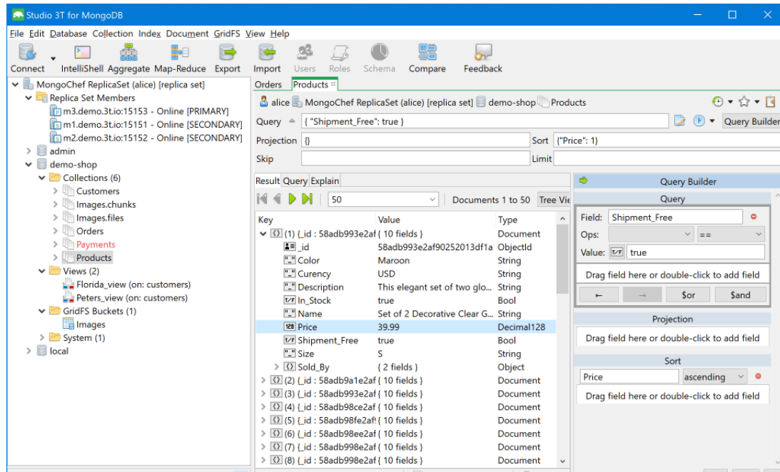
Fig. 5.5: 3T Studio
