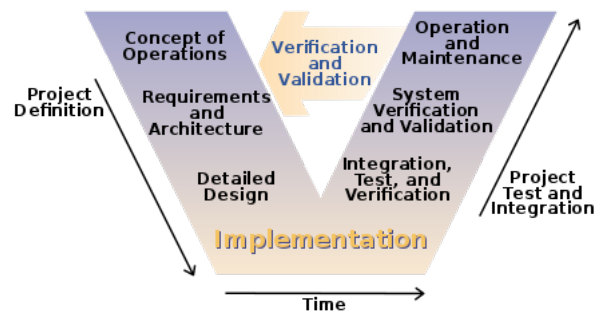
Fig. 3.3: V model
