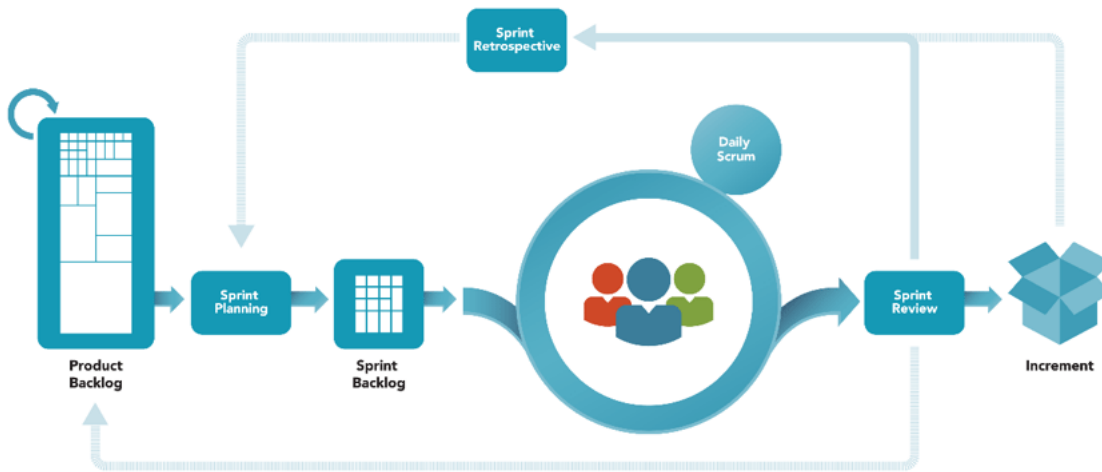
Fig. 3.4: Scrum methodology
