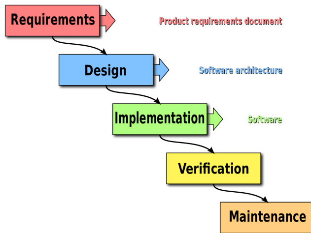
Fig. 3.1: Waterfall methodology
