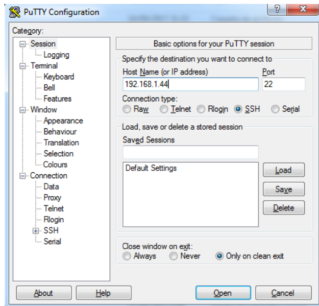
Fig. 5.9: Putty Software
