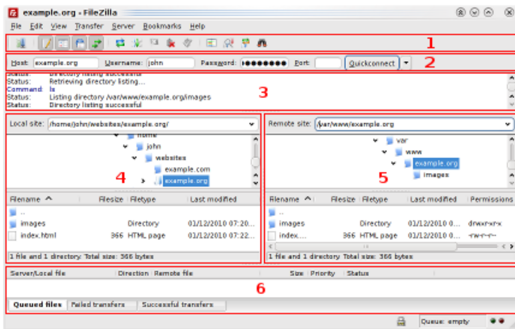
Fig. 5.8: Filezilla's Graphical Interface
