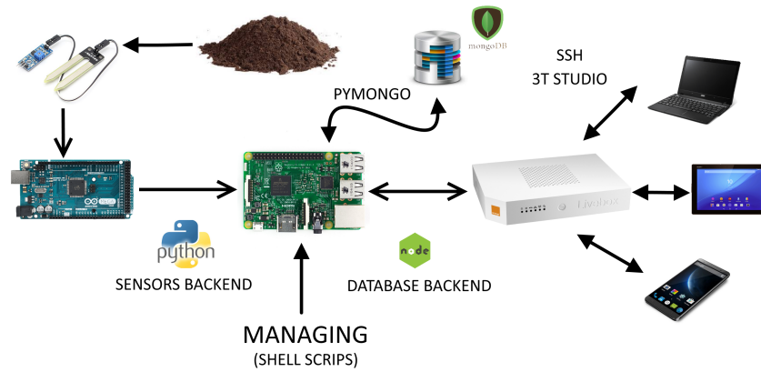
Fig. 4.1: System's architecture
