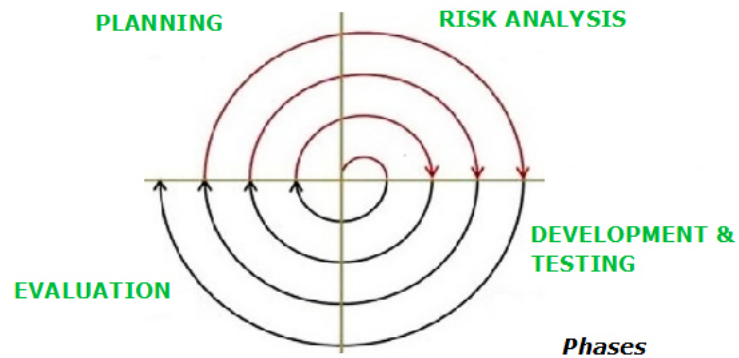
Fig. 3.2: Spiral model
