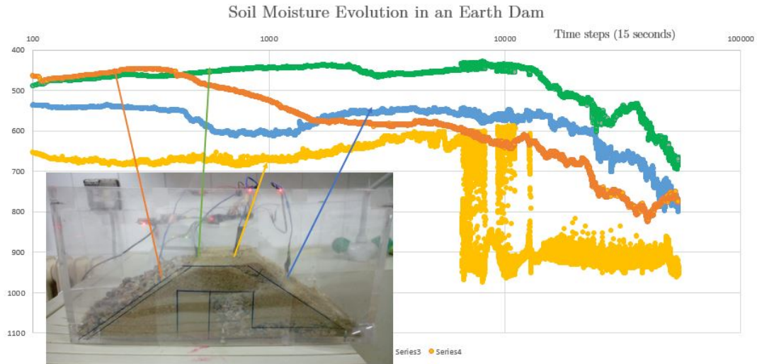
Fig. 6.2: Soil Moisture Evolution in an Earth Dam
