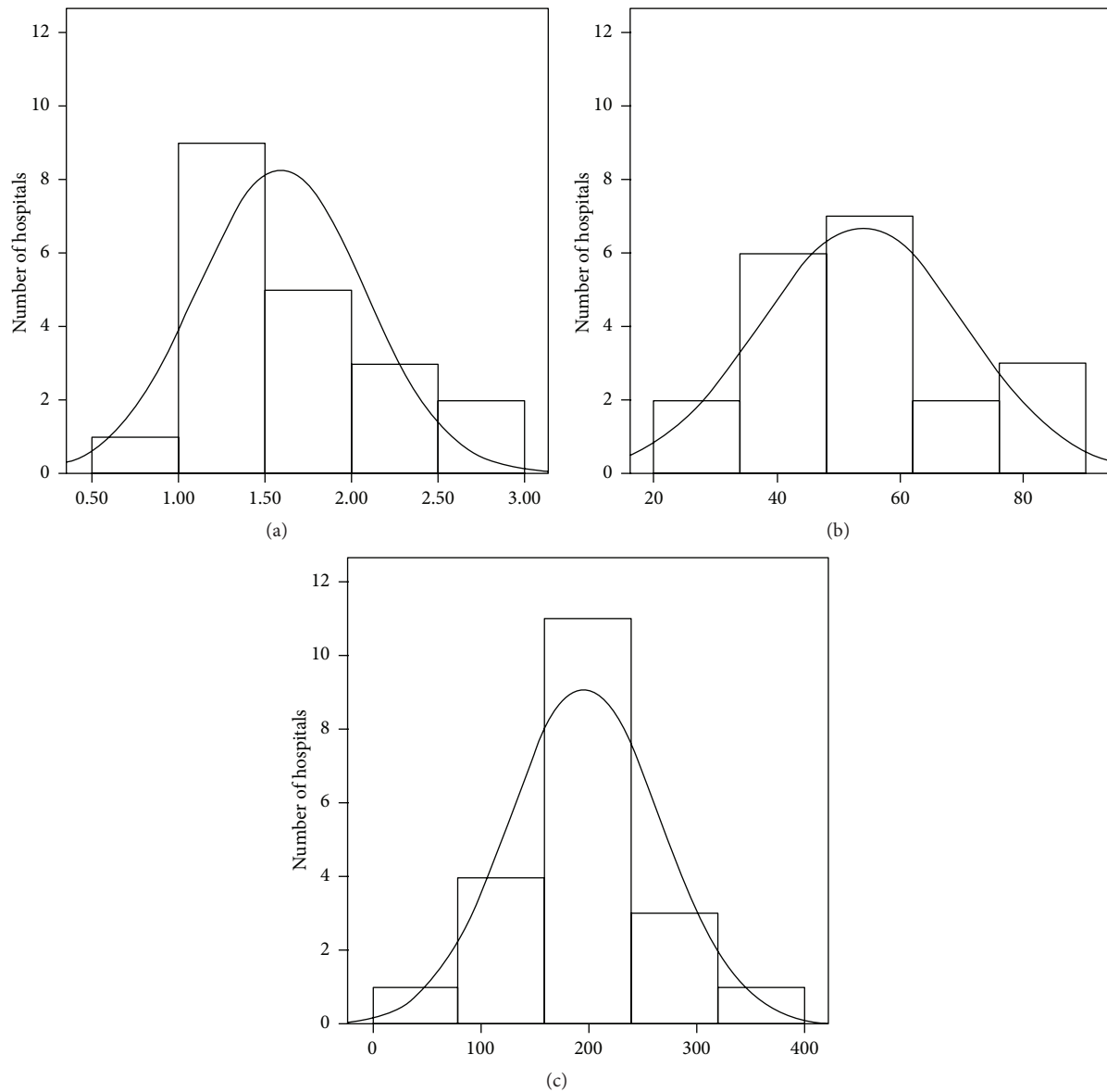
FIGURE 5: Average consumption in \text{m}^3 of CWHC for each indicator: (a) built surface area, (b) number of workers, and (c) number of beds.
