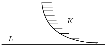
Figure 1: A plane asymptote L of a convex set K .
