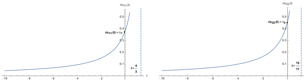
Figure 3: The graphs of \text{ric}_{11}(t) = \text{ric}_{21}(t) and \text{ric}_{12}(t) = \text{ric}_{22}(t) for G_2/U(2) with \mathfrak{m} = \mathfrak{m}_1 \oplus \mathfrak{m}_2 .
