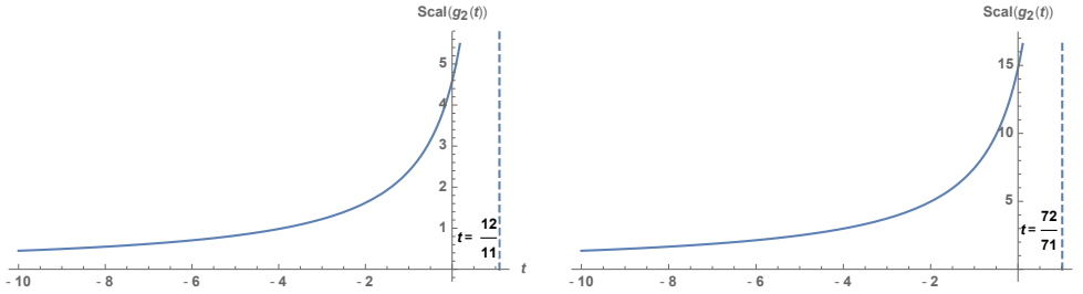
Figure 2: The graph of \text{Scal}(g_2(t)) for G_2/U(2) (left) and F_4/Sp(3) \times U(1) (right).
