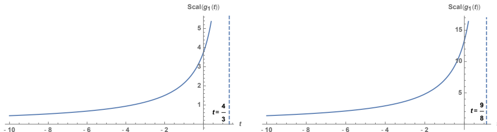
Figure 1: The graph of \text{Scal}(g_1(t)) for G_2/U(2) (left) and F_4/Sp(3) \times U(1) (right).
