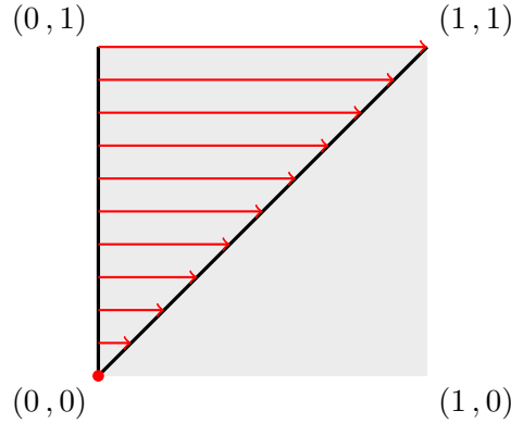
Figure 1: |X| = [0, 1] \times [0, 1] , X^0 = \{0\} \times [0, 1] \cup \{(x, x) : x \in [0, 1]\} , \mathbb{P}_{(0,t),(t,t)}^{\mathcal{G}} X = \mathcal{G}(1, 1) for all t \in ]0, 1[ , \mathbb{P}_{(0,0),(0,0)}^{\mathcal{G}} X = \{(0, 0)\} and \mathbb{P}_{\alpha,\beta}^{\mathcal{G}} X = \emptyset otherwise, there is no composable execution paths.
