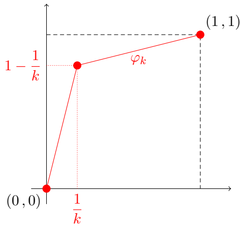
Figure 2: A sequence (\phi_k)_{k \geq 1} of \mathcal{G}(1,1) without limit point
