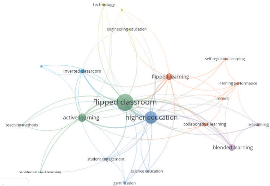
Fig. 5 Cluster mapping
