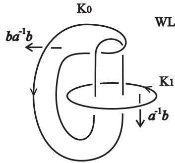
Figure 3: Another planar projection of the Whitehead link.
