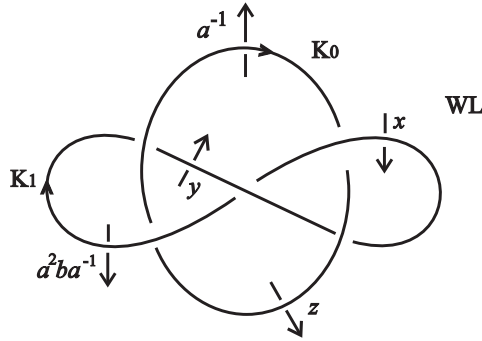
Figure 2: A planar projection of the Whitehead link.
