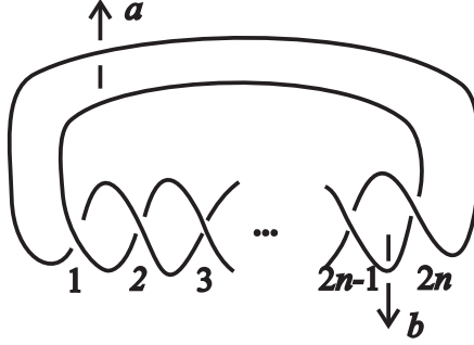
Figure 1: The torus link C(2n) , n \geq 1 .
