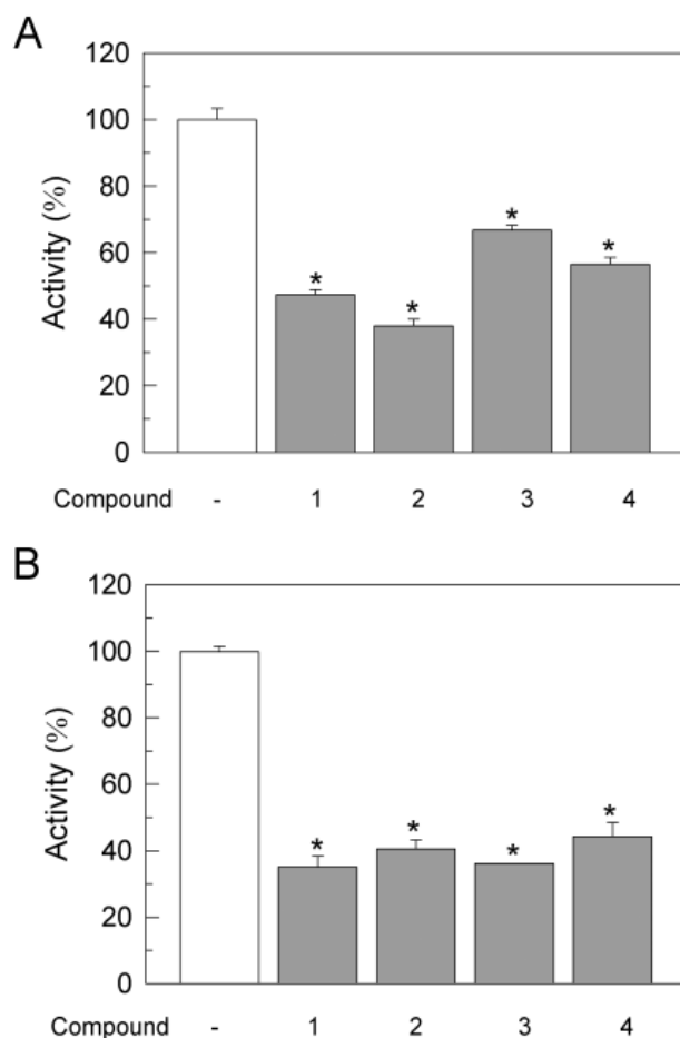
Figure 5. (A) PMCA activity in membrane extracts (10 \mu\text{g} ) from SH-SY5Y cells treated with gold compounds. (B) PMCA activity of non-treated cells before and after addition of compounds to the assay medium, at concentrations of 5, 3, 20, and 1 \mu\text{M} for compounds, 1 , 2 , 3 , and 4 , respectively. Data are expressed as percentage of non-treated cells in the absence of DMSO, as mean \pm SEM of at least three independent experiments carried out in triplicate with three different cultures. Symbols (*) represent significant differences when compared to control (ANOVA, Dunnett's test, p < 0.05 ).
