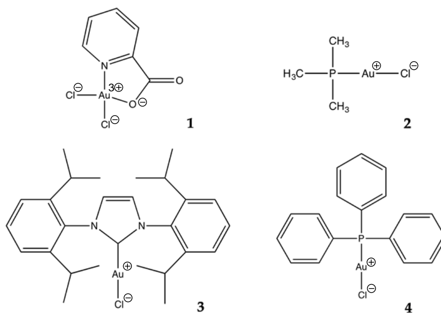
Figure 1. Structures of the gold complexes used in the study: (1) dichloro (2-pyridinecarboxylate) gold(III); (2) chlorotrimethylphosphine gold(I); (3) 1,3-bis(2,6-diisopropylphenyl) imidazole-2-ylidene gold(I) chloride; and (4) chlorotriphenylphosphine gold(I). Formal charge distribution is also shown.
