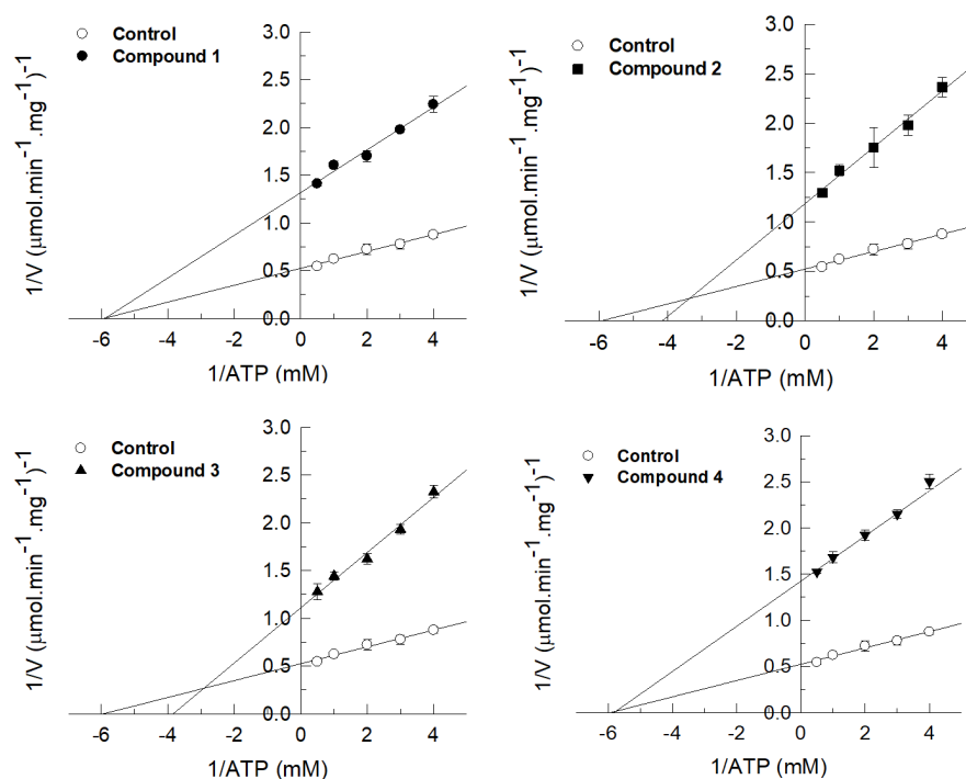
Figure 3. Lineweaver–Burk plots of \text{Ca}^{2+} -ATPase activity in the absence (empty symbols) and in the presence (filled symbols) of gold compounds 1, 2, 3, and 4, at concentrations of 5, 3, 21, and 1 \mu\text{M} , respectively. The plots were used to determine the type of PMCA inhibition. The gold complexes 1 and 4 presented a non-competitive type of inhibition, while compounds 2 and 3 showed a mixed type of inhibition. Data are plotted as means \pm standard deviation. The results shown are the average of triplicate experiments carried out in distinct preparations.
