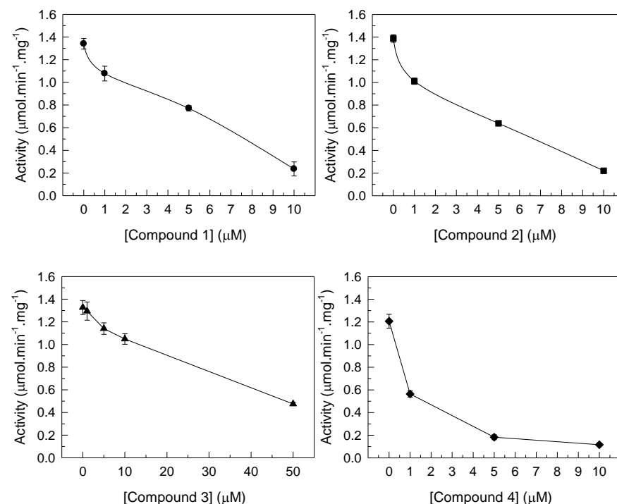
Figure 2. Inhibition of PMCA activity by gold compounds 1, 2, 3, and 4. The Ca^{2+} -ATPase was measured spectrophotometrically at 340 nm and 37 °C, using the coupled enzyme pyruvate kinase/lactate dehydrogenase assay. The experiments were initiated after the addition of 2.5 \mu g/mL of purified PMCA reconstituted in PCIIS. Data are plotted as means \pm SD. The results shown are the average of triplicate experiments carried out with different preparations.
