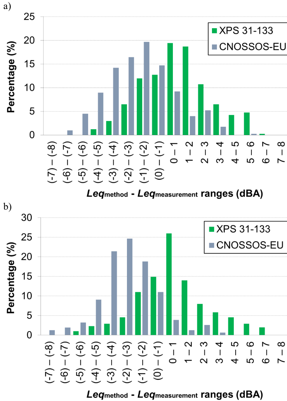
Fig. S2. Distribution of noise model uncertainties in cities of (a) Talca and (b) Moraleja
