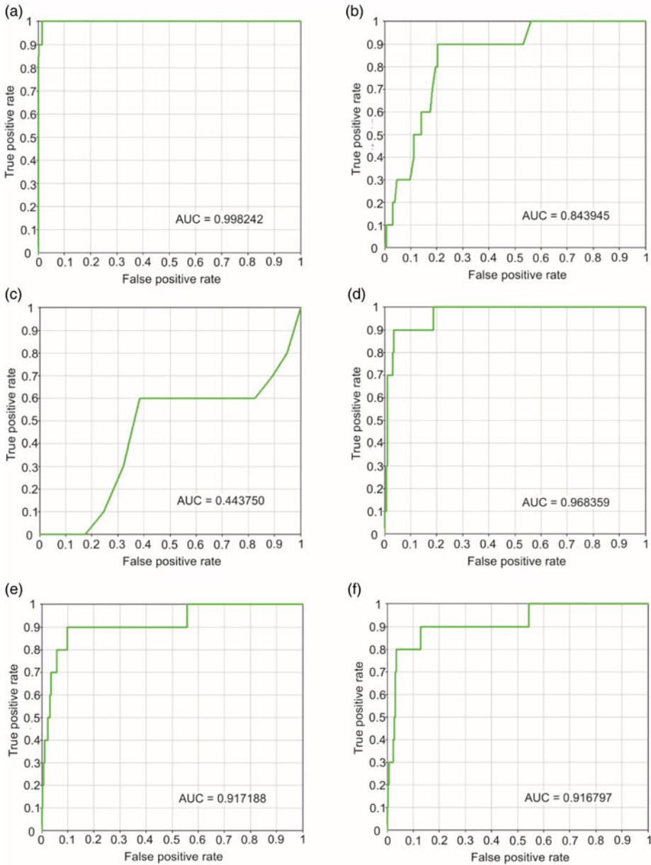
Figure 3. ROC curves and AUCs using different algorithms for Rwy<2,500: (a) Greedy Thick Thinning; (b) Bayesian Search; (c) Essential Graph Search; (d) Tree Augmented Naive Bayes; (e) Augmented Naive Bayes; (f) Naive Bayes.
