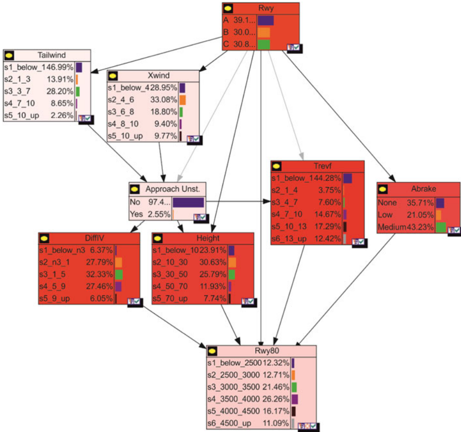
Figure 4. Graphical representation of the BN considered.
