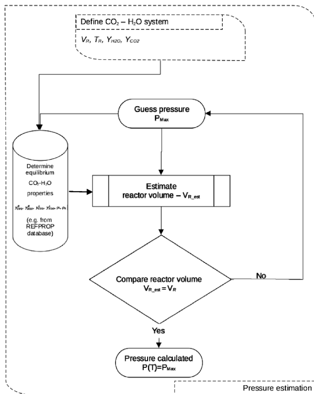
Fig. 2. Flow diagram of the algorithm to estimate pressure in the reactor using the CO 2 -H 2 O properties under HTC conditions.
