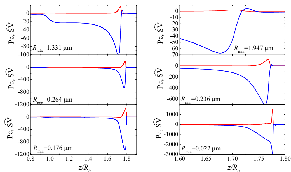
Figure 6. Axial distribution of the capillary pressure P_c (blue lines) and normal shear viscous stress \widehat{S_V} (red lines) for DIW+SDS 0.8cmc and three instants as indicated by the value of R_{\min} . The left-hand and right-hand graphs correspond to \{\mu_1^{S*} = 5 \times 10^{-9}, \mu_2^{S*} = 0 \text{ Pa s m}\} and \{\mu_1^{S*} = 1.2 \times 10^{-9}, \mu_2^{S*} = 0 \text{ Pa s m}\} , respectively. The results were calculated for B = 3.396 \times 10^{-3} , Oh = 0.0151 , \Gamma_{\text{cmc}} = 1.002 , Pe^S = 7.730 \times 10^4 , Oh_2^{S*} = 0 , and Oh_1^{S*} = 6.563 \times 10^{-4} (left-hand graphs) and 1.575 \times 10^{-4} (right-hand graphs) (see “Methods” section).
